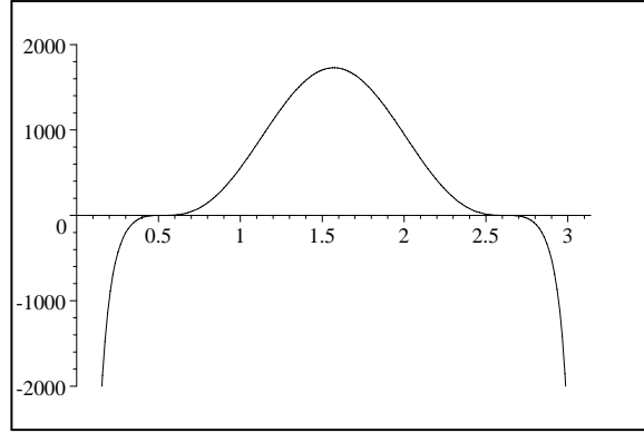
Fig 2. j -invariant in the complex Case II
