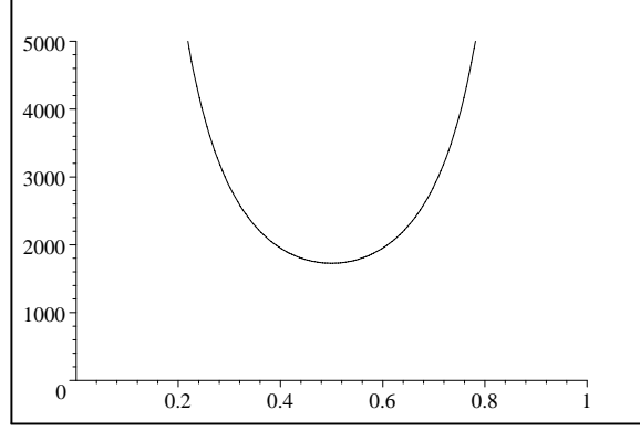
Fig 1. j -invariant in the real Case I
