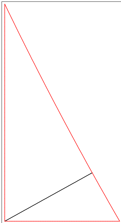
Figure 9: Billiard from cba
