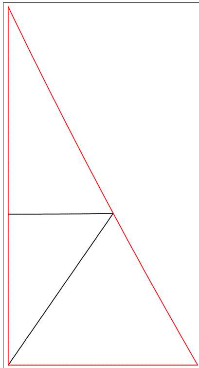
Figure 10: Billiard from cbababba
