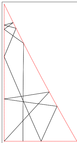
g = pqrpqrpqrprpqrpqrprpqrpqrpr, l_w(g) = 23 billiard length: 3.799186511
