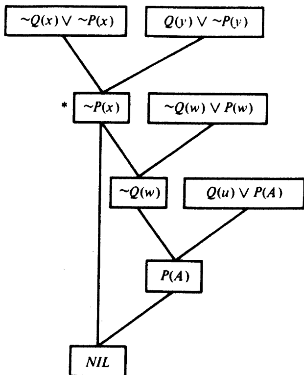
Fig. 5.5 A refutation tree.
