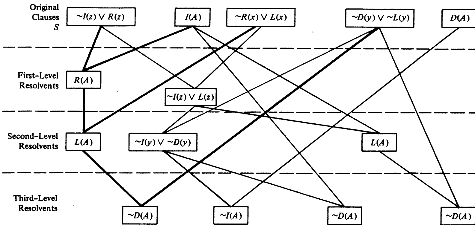
Fig. 5.3 Illustration of a set-of-support strategy.
