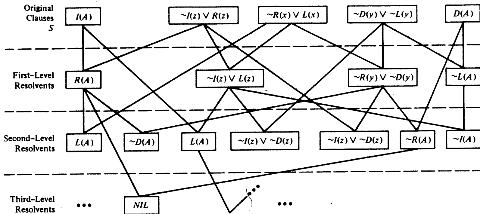
Fig. 5.2 Illustration of a breadth-first strategy.
