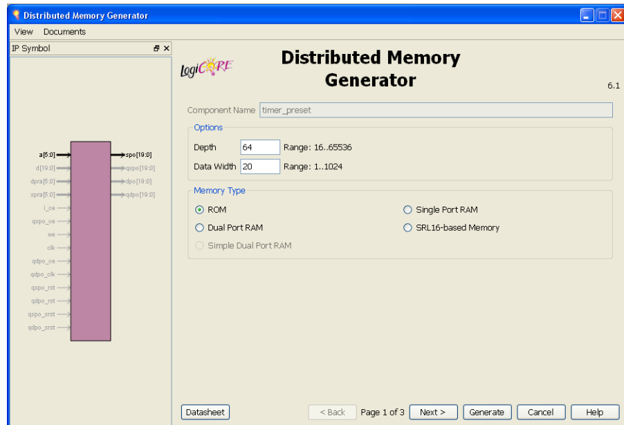
Figure 3-12: CORE Generator Tool—Distributed Memory Generator Customization GUI Page 1
