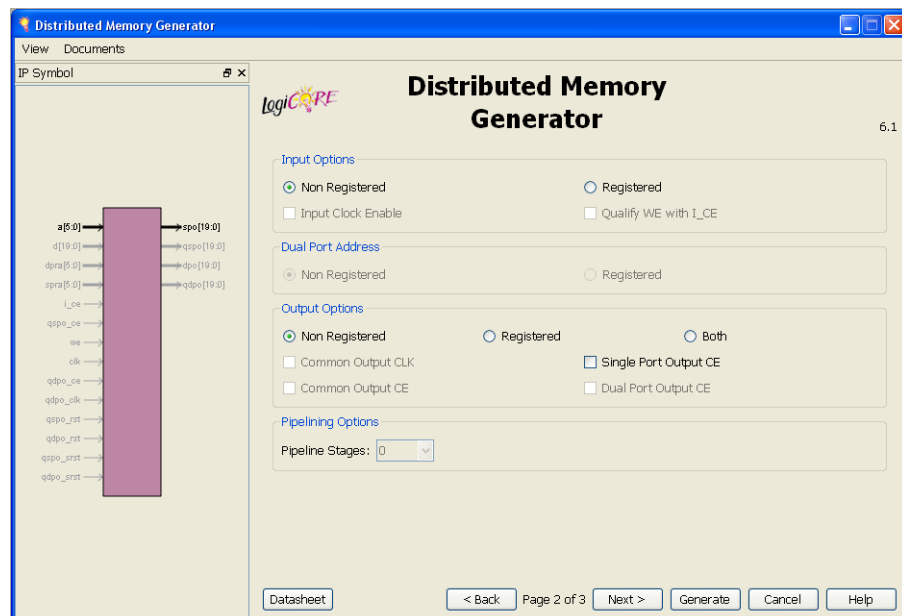
Figure 3-13: CORE Generator Tool—Distributed Memory Generator Customization GUI Page 2
