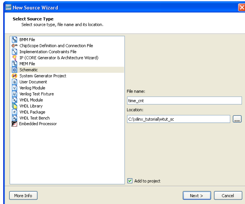
Figure 4-4: New Source Dialog Box
