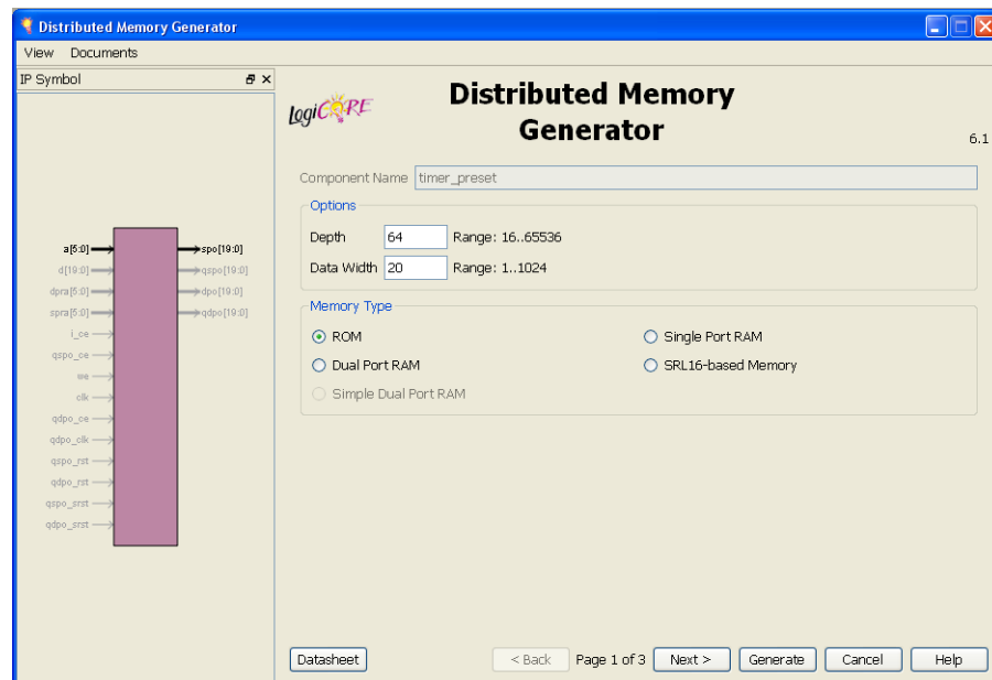
Figure 4-17: CORE Generator Tool—Distributed Memory Generator Customization GUI
