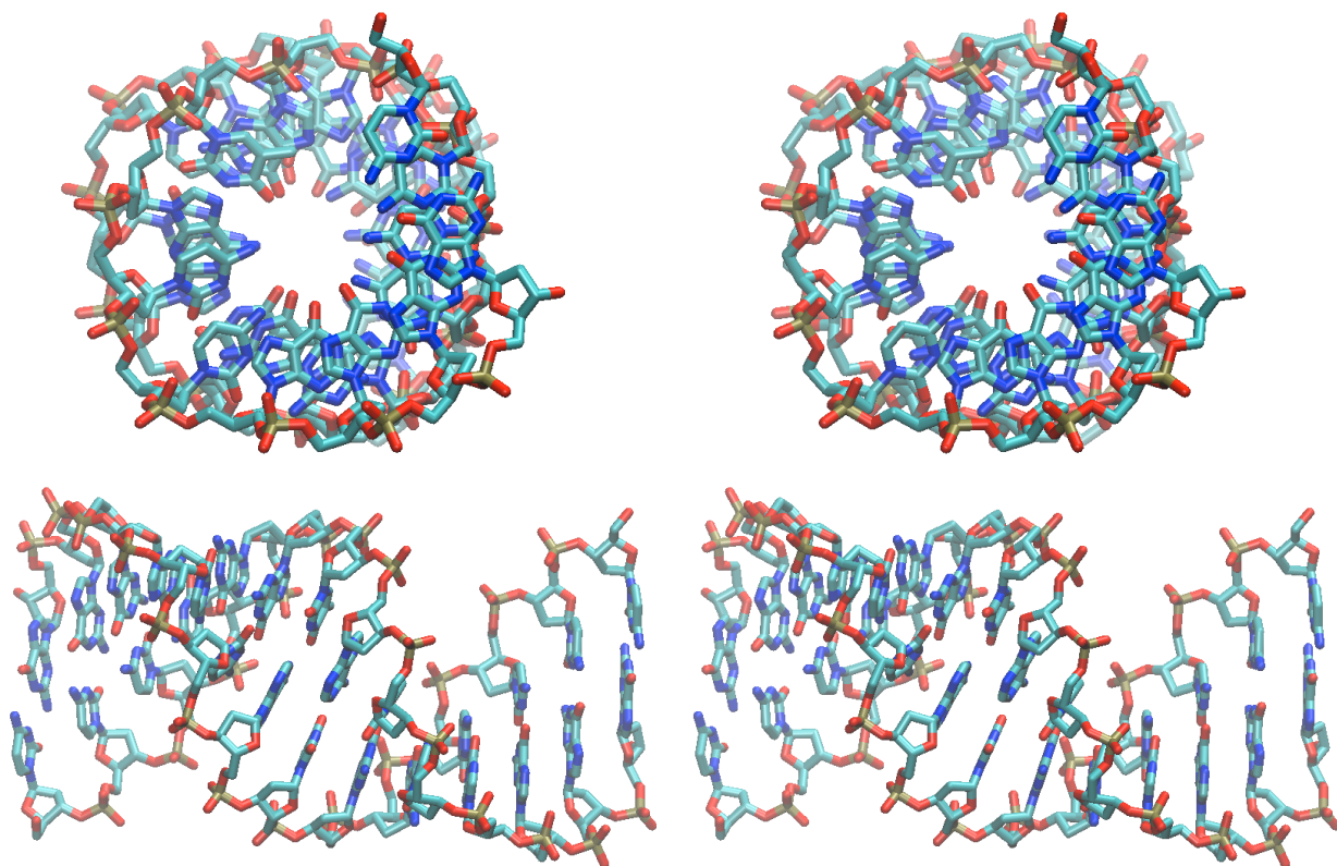
Stereoview of A-Form DNA (from pdb ID 3V9D)
