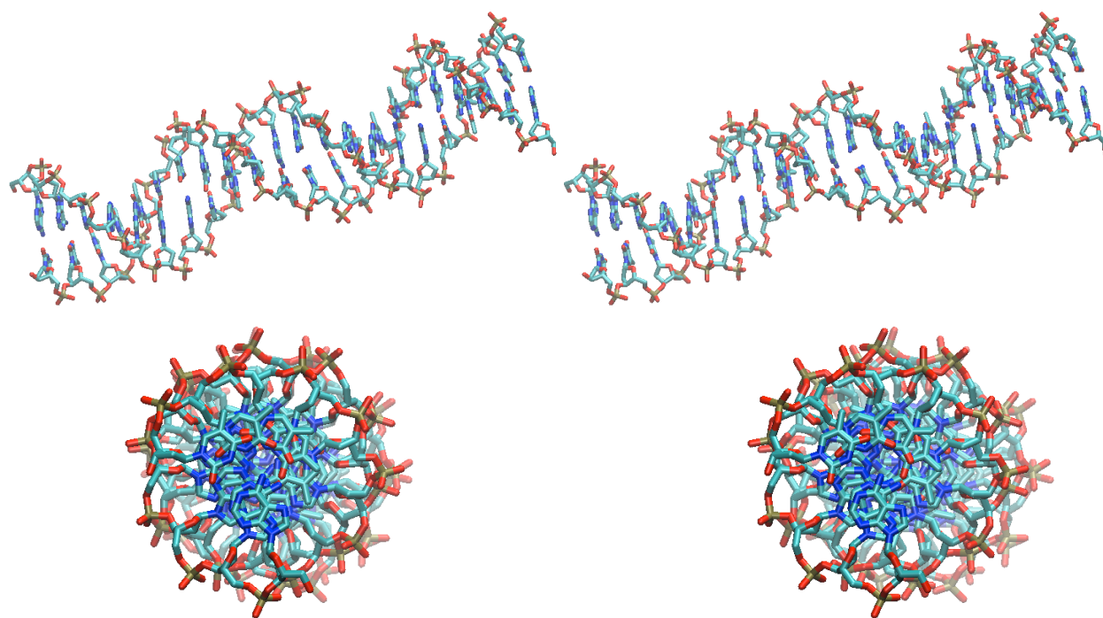
Stereoview of B-Form DNA (from pdb ID 1A36)
