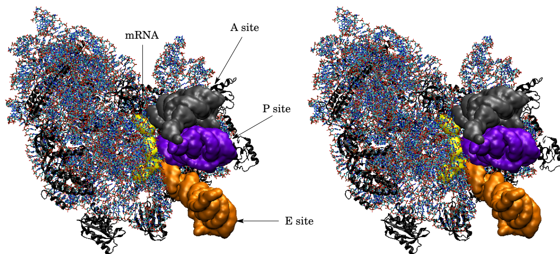
Stereoview of Thermus thermophilus 30 S ribosome subunit (pdb ID 2wdk)
