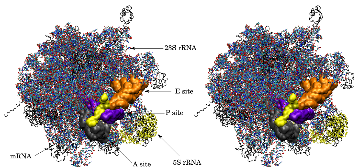
Stereoview of Thermus thermophilus 50 S ribosome subunit (pdb ID 2wdl), with mRNA and tRNA from pdb ID 2wdk
