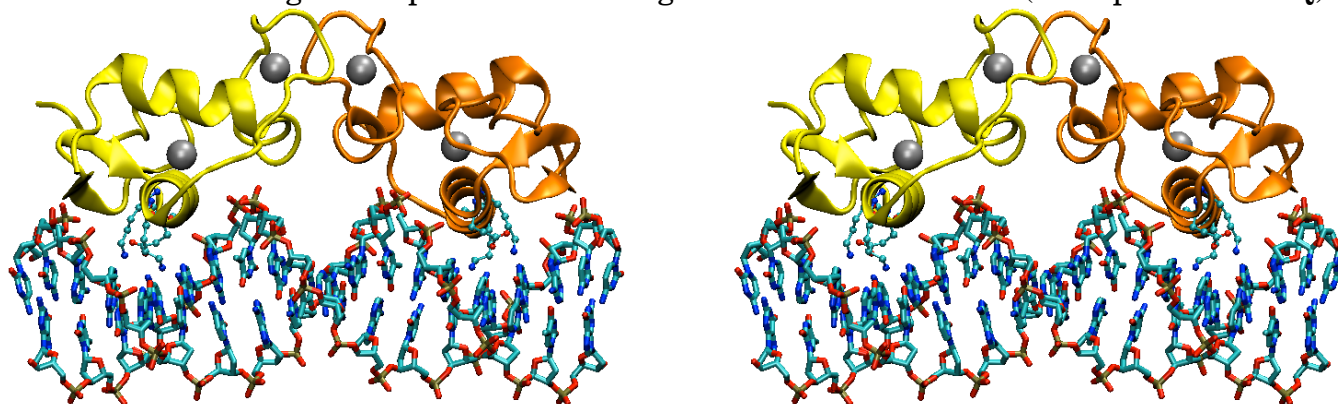
Stereoview of estrogen receptor DNA-binding domain bound to DNA (from pdb ID 1HCQ)
