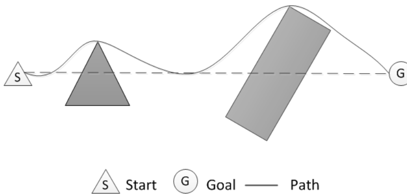
Figure 4: Tangent Bug Obstacle Avoidance
