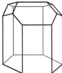
Figure 5: A half elongated rhombic dodecahedron, described by Fejes Tóth [FT2], is the conjectured surface-area-minimizing 10-hedral tile. Image from [FT2].
