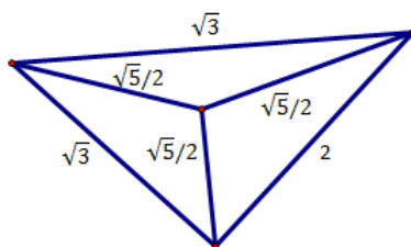
Figure 17: No. 3 tetrahedron is given by cutting a square pyramid into two. [So, Fig. 9].
