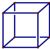
Figure 3: A cube is the surface-area-minimizing 6-hedron.
