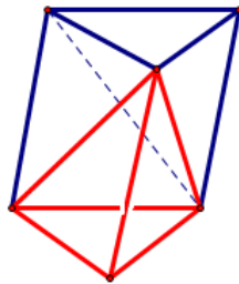
Figure 1: A tetrahedron formed by cutting a triangular prism into three congruent tetrahedra is the conjectured surface-area-minimizing tetrahedral tile.
