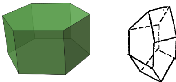
Figure 4: A hexagonal prism [Wi] and Goldberg’s [G7, Fig. 8-VI] gabled rhombohedron are the conjectured surface-area-minimizing 8-hedral tiles. They have the same surface area.
