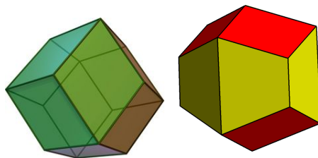
Figure 7: A rhombic dodecahedron and a trapezo-rhombic dodecahedron are the conjectured surface-area-minimizing 12-hedral tiles. They have the same surface area. Images from [Wi].
