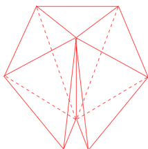
Figure 10: Because the dihedral angles ( 70.53^\circ ) of a regular tetrahedron cannot add up to 360^\circ , the regular tetrahedron does not tile; there is a small gap. Image from [U].
