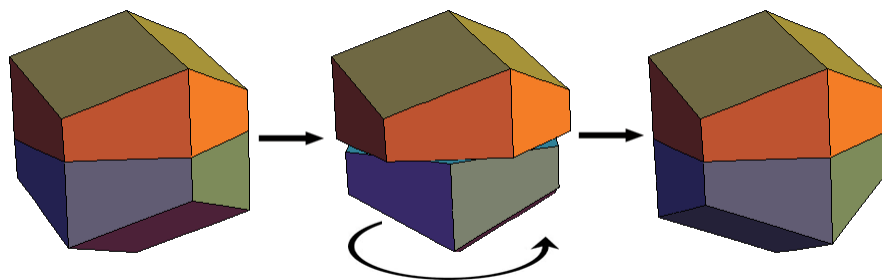
Figure 13: Rotating half of a rhombic dodecahedron yields the trapezo-rhombic dodecahedron. Images from [Haf1].
