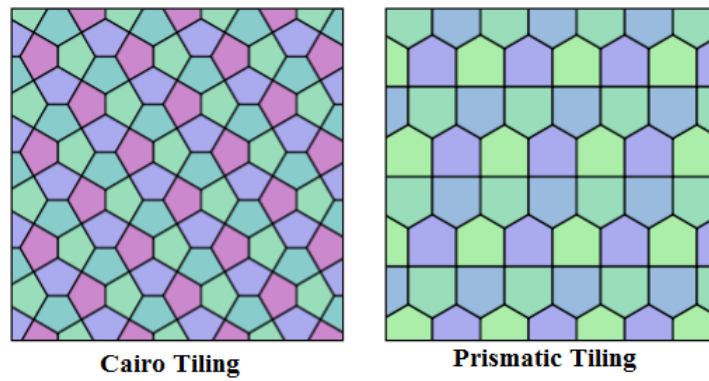
Figure 11: Cairo and Prismatic pentagons have recently been proved as the best pentagonal planar tiles (Chung et al. [CFS, Thm. 3.5]). Image from [Wi].
