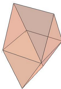
Figure 12: The optimal Schmitt-Conway biprism [Wei] is an 8-hedron with surface area greater than that of the cube. Image from [Haf2].
