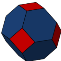
Figure 9: Kelvin's truncated octahedron is the conjectured surface-area-minimizing convex polyhedral tile. Image from [Wi].
