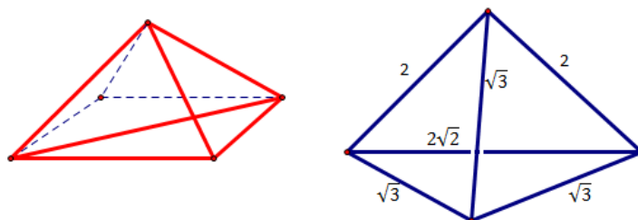
Figure 16: No. 2 tetrahedron is given by cutting No. 3 in half. [So, Fig. 8].
