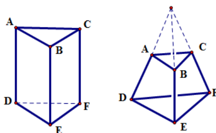
Figure 19: In a combinatorial triangular prism, the lines AD , BE , and CF are either parallel to each other or concur at a point.
