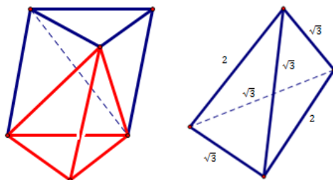
Figure 15: The tetrahedron (Sommerville No. 1) formed by four isosceles triangles with two sides of \sqrt{3} and one side of 2 minimizes surface area among all orientation-preserving tetrahedral tiles [So, Fig. 7].
