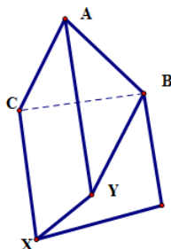
Figure 14: Two triangular faces cannot meet in a nondegenerate polyhedron with three quadrilateral faces and two triangular faces.
