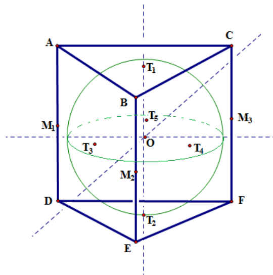
Figure 21: A right equilateral-triangular prism circumscribed about a sphere tangent to each face at its centroid minimizes surface area among unit-volume 5-hedra.
