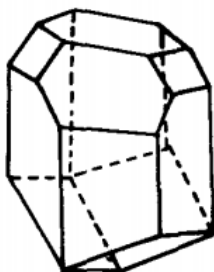
Figure 8: Combining half of the bee cell and half of a Fejes Tóth Cell yields our conjectured surface-area-minimizing 13-hedral tile. Image from [G1].
