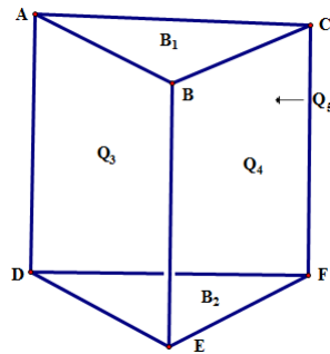
Figure 20: By Proposition 5.7, the surface-area-minimizing 5-hedron X cannot be a square pyramid; therefore by Proposition 5.4, X is a combinatorial triangular prism.
