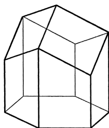
Figure 4: A hexagonal prism [Wi] and Goldberg’s [G7, Fig. 8-VI] gabled rhombohedron are the conjectured surface-area-minimizing 8-hedral tiles. They have the same surface area.
