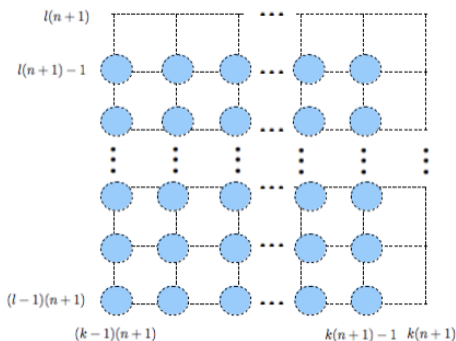
Figure 3: I_{k,l}^{(n)}
