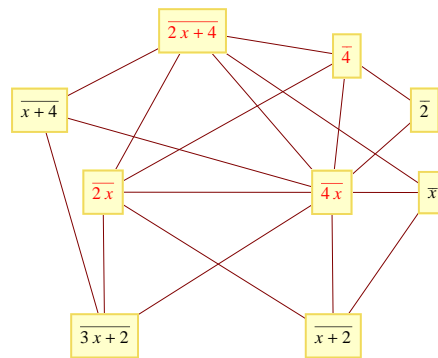
Figure 4: \Gamma_c(\mathbb{Z}_8[x]/(x^2 + 2x))
