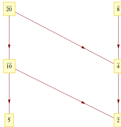
Figure 8: \Lambda(\mathbb{Z}_{40})
