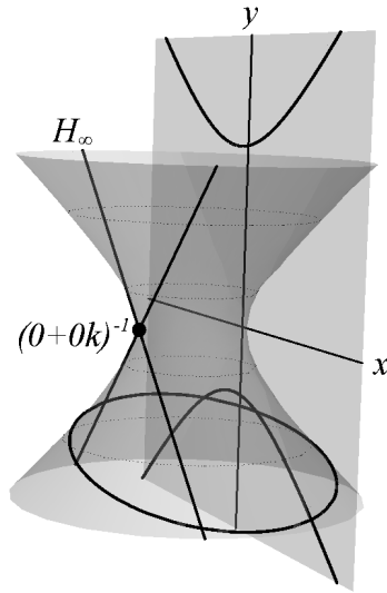
FIGURE 5. Representation of a hyperbola on the hyperboloid projected onto the double plane
