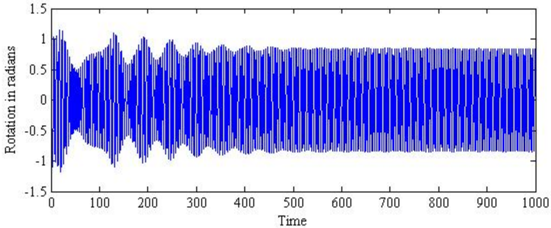
Figure 3.2-6—The bridge response with \lambda_2 = -0.025 for S = 50 and E = 61.4
