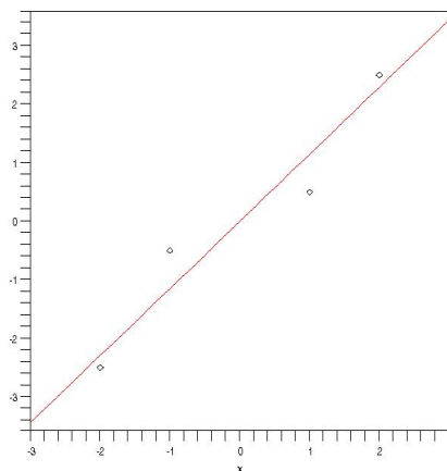
Figure 2: The Columns of Q_{sub} Plotted as Points with the One-Dimensional Subspace Spanned by the First Eigenvector of Q_{sub} * Q_{sub}^T
