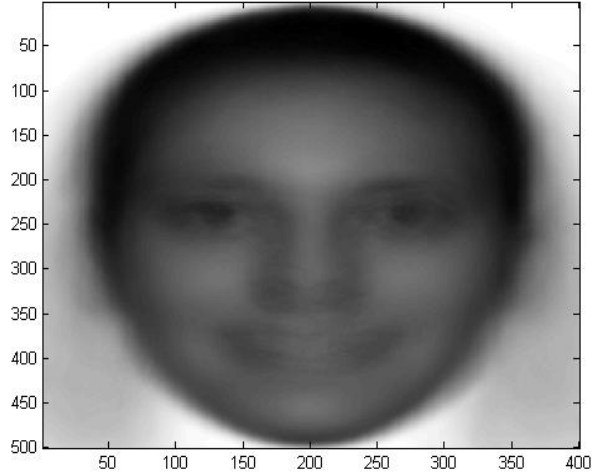
Figure 3: Average Face from First Database
