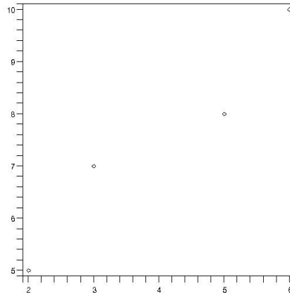
Figure 1: Vectors formed by the Columns of Q Plotted as Points in the Euclidean Plane
