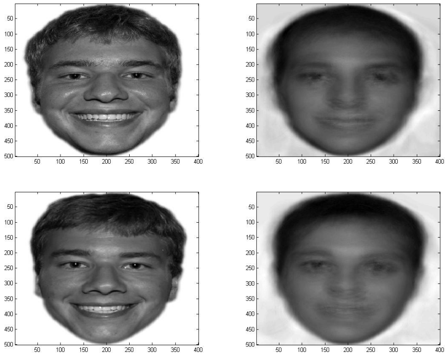
Figure 7: The top two images are the original face and the fifteen vector approximation of one of the brothers. The bottom two are the original face and the fifteen vector approximation of the other brother.
