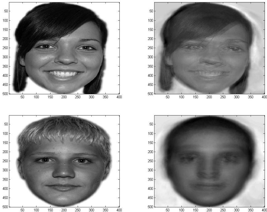
Figure 6: The top two are the original face and the fifteen vector approximation of the face that can be best approximated. Similarly, the bottom two are the original face and the fifteen vector approximation of the face that is most inaccurately approximated.
