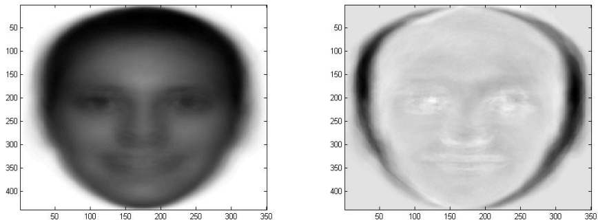
Figure 8: The image on the left is the average face from the second database, and the image on the right is the first eigenface from this database.
