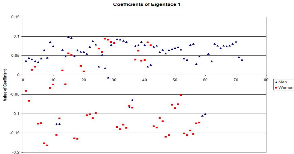
Figure 5: Coefficients of Eigenface 1 for each Face based on Gender
