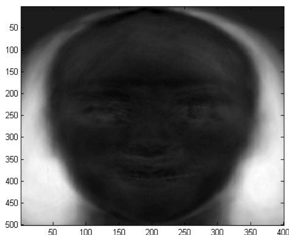
Figure 4: First Eigenface from Database 1
