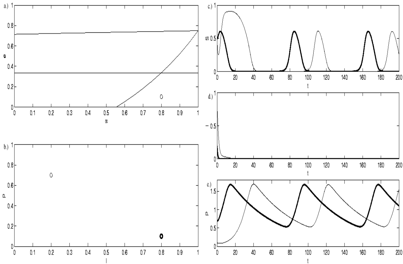
Figure 5: Graphs describing the dynamics in region 6. All parameter and initial condition values are the same as the previous cases. Only the point (\alpha, e) has been modified to be (0.8, 0.1) .
