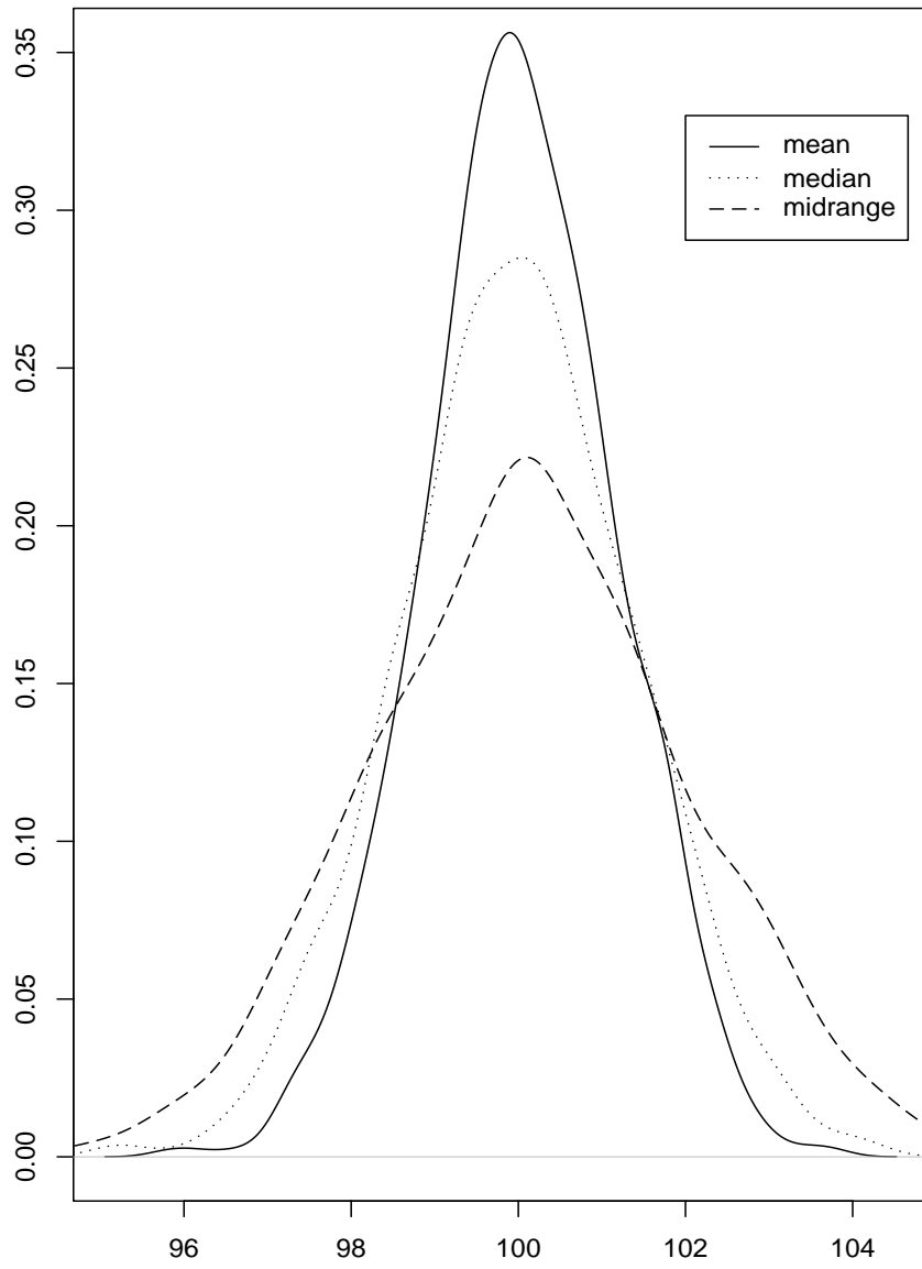
Figure 3.1.3: Normal Distribution 2
