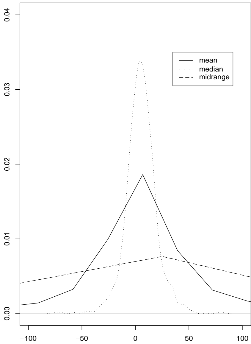
Figure 3.2.2: Cauchy Distribution 1
