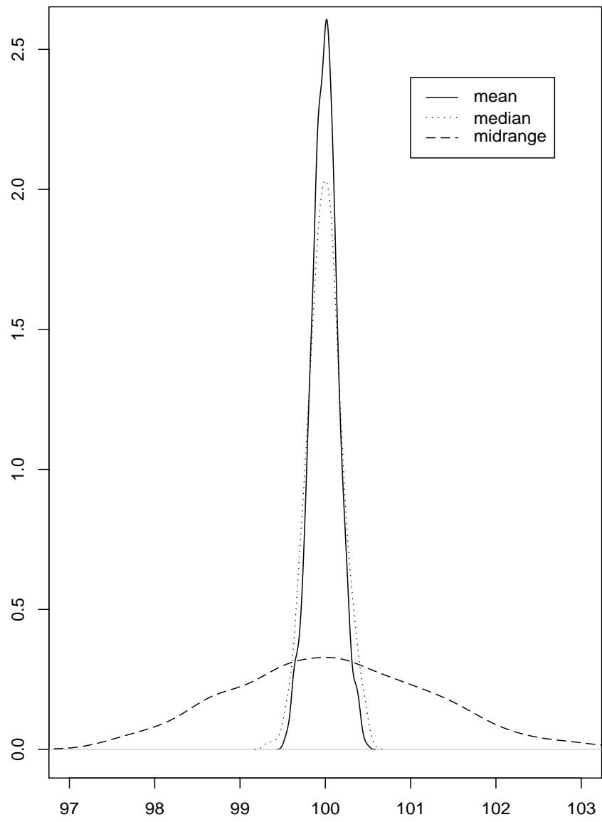
Figure 3.1.5: Normal Distribution 4
