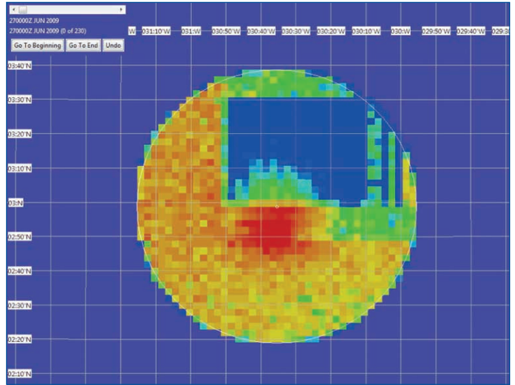
Figure 12: Posterior PDF after Phase 1.
