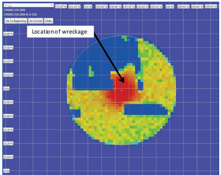
Figure 5. Posterior PDF assuming pingers failed.
