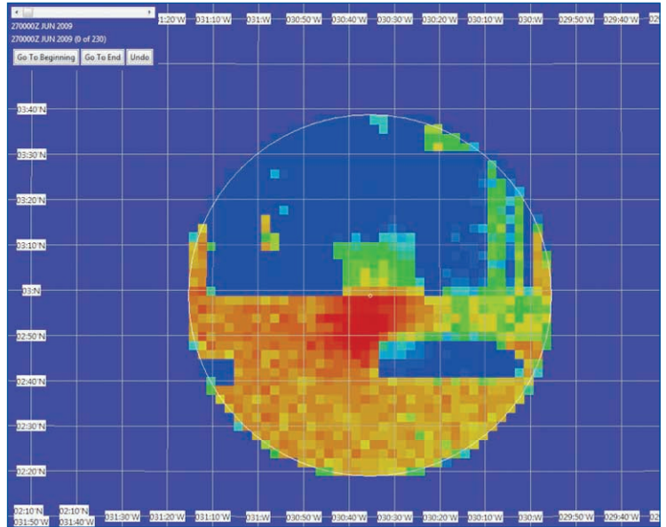
Figure 4: Posterior PDF after Phase 3. Red cells indicate high probabilities. Decreasing probabilities are shown by orange to yellow to green to blue cells.
