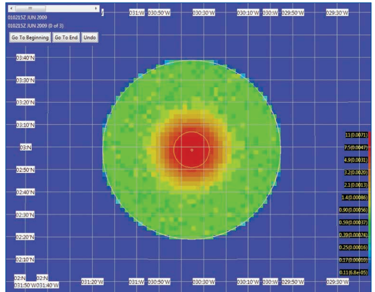
Figure 8: Flight dynamics prior.
