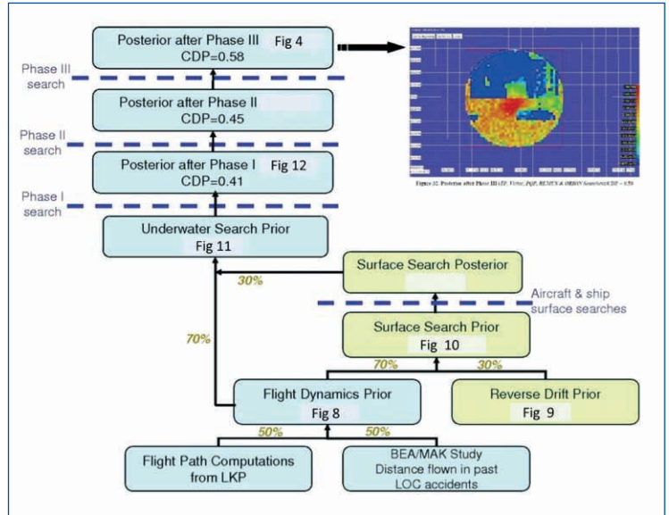
Figure 7. Summary of PDF computation.
