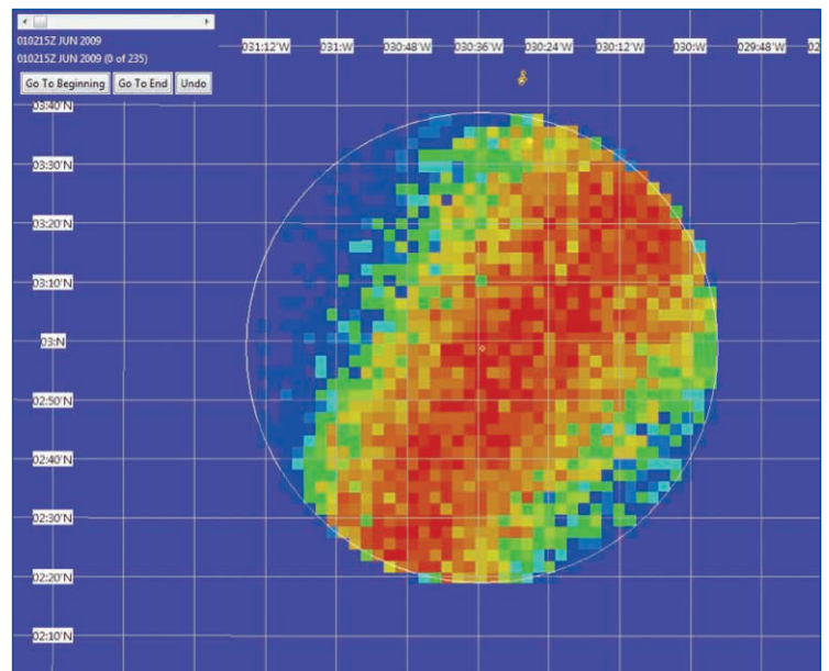
Figure 9: Reverse drift PDF.
