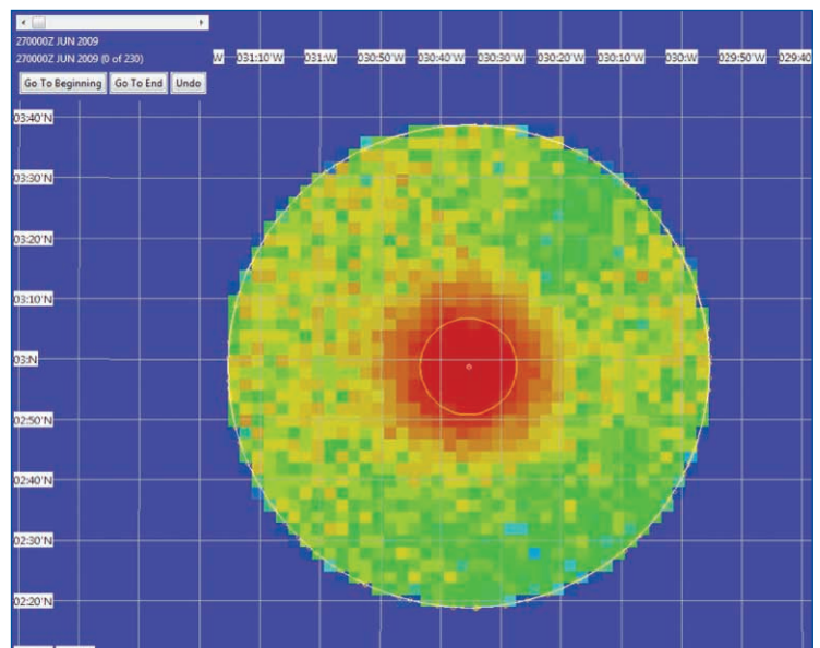
Figure 11: Underwater search prior.
