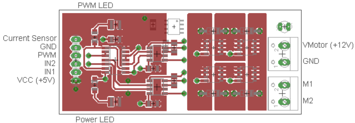
Figure 5. H Bridge connections
