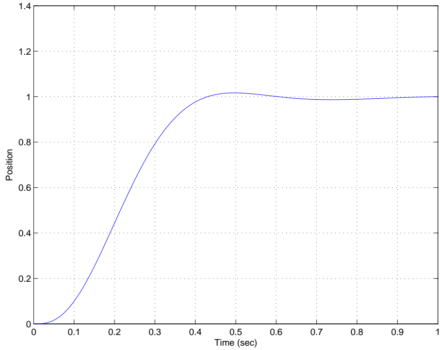
Figure 22: The unit step response of the third order deadbeat system from Example 5 ( \omega_0 = 10 rad/sec.)
