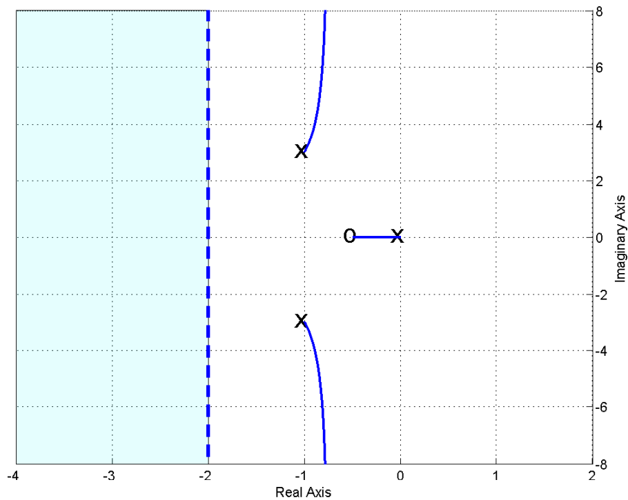
Figure 47: Root locus plots for G_p(s) = \frac{2}{s^2+2s+10} with the proportional+integral (PI) controllers with the controller zero at -3 (top) and -0.5 (bottom). To match the settling time all poles must be to the left of -2.
