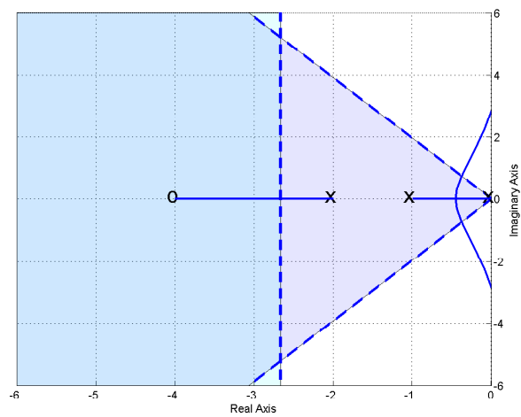
Figure 56: Root locus plot for G_p(s) = \frac{2}{s^2+3s+2} with three proportional+integral (PI) controllers. None of these systems will ever meet the settling time criteria. All three will meet the percent overshoot criteria if k is small enough. The third system will become unstable for k sufficiently large.
