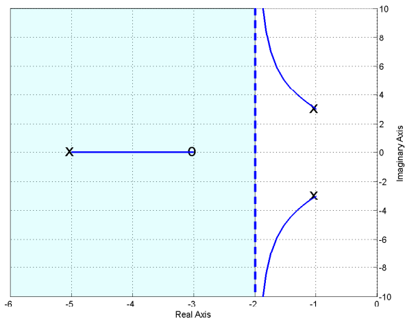
Figure 51: Root locus plots for G_p(s) = \frac{2}{s^2+2s+10} with lead controllers for l = 2 and asymptote \sigma_c = -2 . To match the settling time all poles must be to the left of -2.
