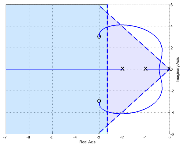
Figure 60: Root locus plots for G_p(s) = \frac{2}{s^2+3s+2} with proportional+integral+derivative (PID) controllers with complex conjugate zeros. The systems in the top two panels demonstrate bad choices for the location of the controller zeros.
