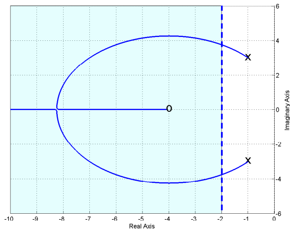
Figure 48: Root locus plots for G_p(s) = \frac{2}{s^2+2s+10} with the proportional+derivative (PD) controllers with the controller zero at -1 (top), -2 (middle), and -4 (bottom). To match the settling time all poles must be to the left of -2.
