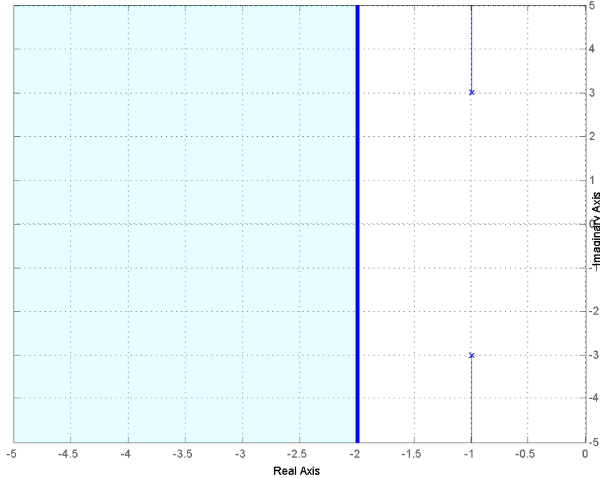
Figure 45: Root locus plot for G_p(s) = \frac{2}{s^2+2s+10} with the proportional (P) controller. To match the settling time all poles must be to the left of -2.
