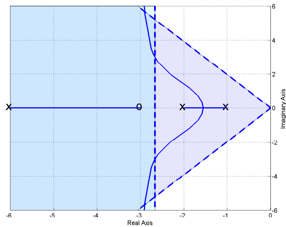
Figure 62: Root locus plots for G_p(s) = \frac{2}{s^2+3s+2} with lead controllers. Here l = 3 for all three controllers. However, only the third system is capable of meeting both the settling time and percent overshoot criteria. If k becomes too large in these systems the percent overshoot criteria will not be met.
