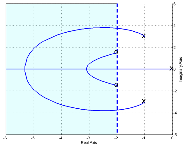
Figure 65: Root locus plot for G_p(s) = \frac{2}{s^2+2s+10} with the pid controller as the imaginary part of the zeros move closer to the real axis. This graph exemplifies some of the possible root locus behavior we have not seen yet. To match the settling time all poles must be to the left of -2.
