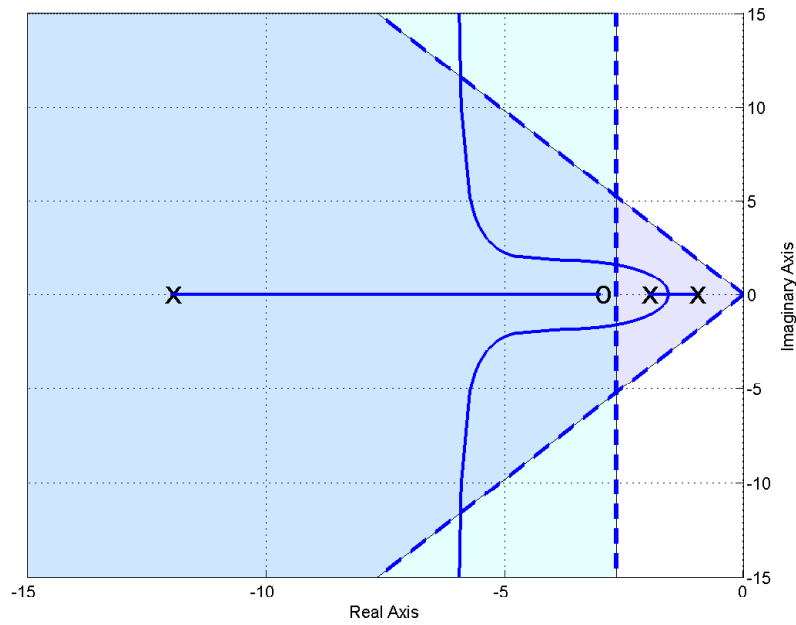
Figure 63: Root locus plots for G_p(s) = \frac{2}{s^2+3s+2} with lead controllers. Here l = 6 (top panel) and l = 9 (bottom panel). If k becomes too large in these systems the percent overshoot criteria will not be met.
