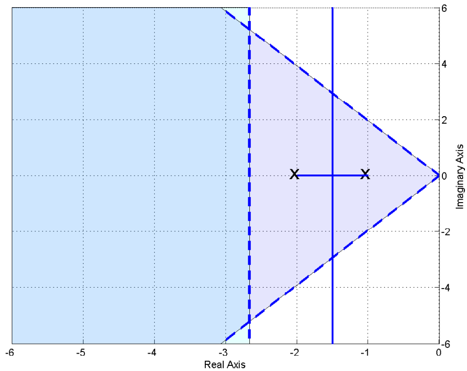
Figure 54: Root locus plot for G_p(s) = \frac{2}{s^2+3s+2} with the proportional (P) controller. This system will never meet the settling time criteria, but it will meet the percent overshoot criteria as long as k is not too large.
