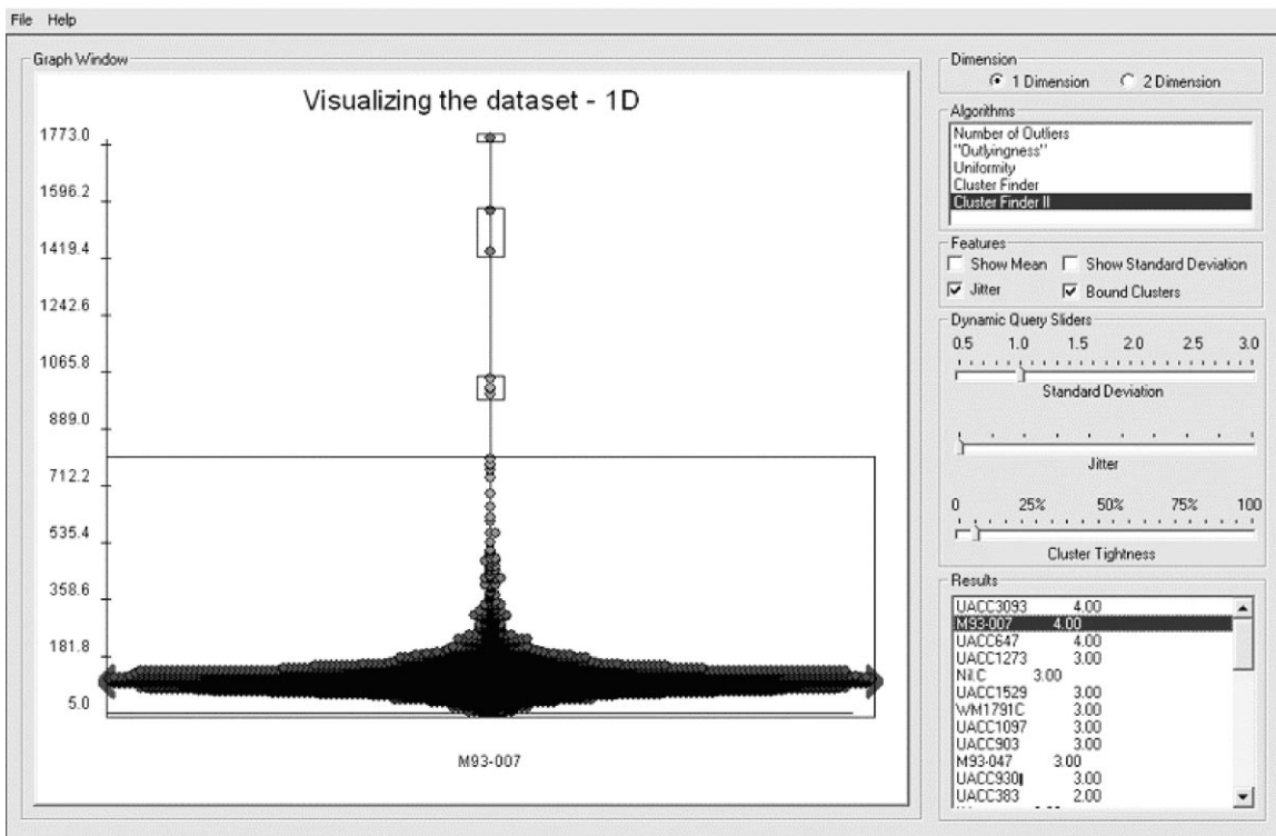
Figure 4 Prototype panel to enable user specification of 1-dimensional distribution requirements. User has chosen the Cluster Finder II algorithm that ranks all distributions according to the number of identifiable clusters, while allowing users to specify Cluster Tightness with a slider (Implemented by Kartik Parija and Jaime Spacco).
