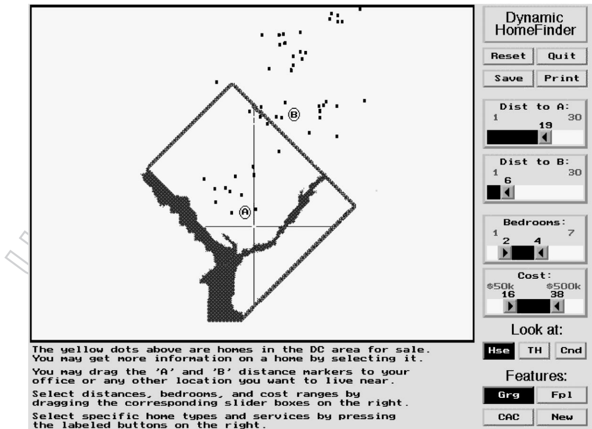
Figure 2 Dynamic Queries HomeFinder with sliders to control the display of markers indicating homes for sale. Users can specify distances to markers, bedrooms, cost, type of house and features 15 .
