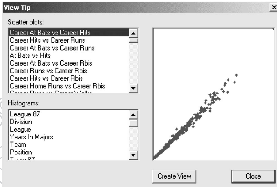
Figure 3 Spotfire View Tip panel with ranking of possible 2-dimensional scatter plots in descending order by the strength of linear correlation. Here the strong correlation in baseball statistics is shown between Career At Bats and Career Hits. Notice the single outlier in the upper right corner, representing Pete Rose's long successful career.
