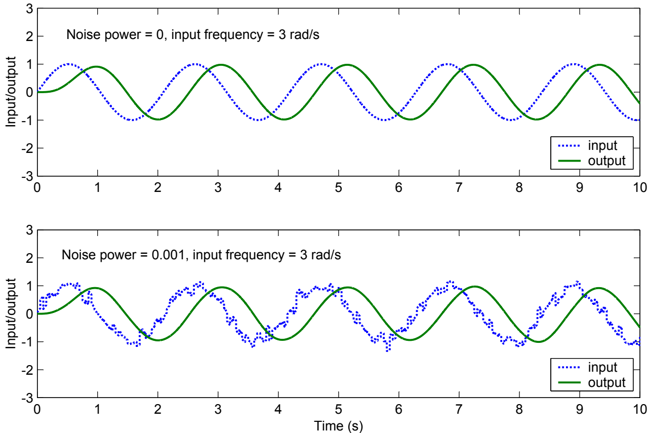
Fig.1: Filter output with a constant input frequency and different levels of noise.
