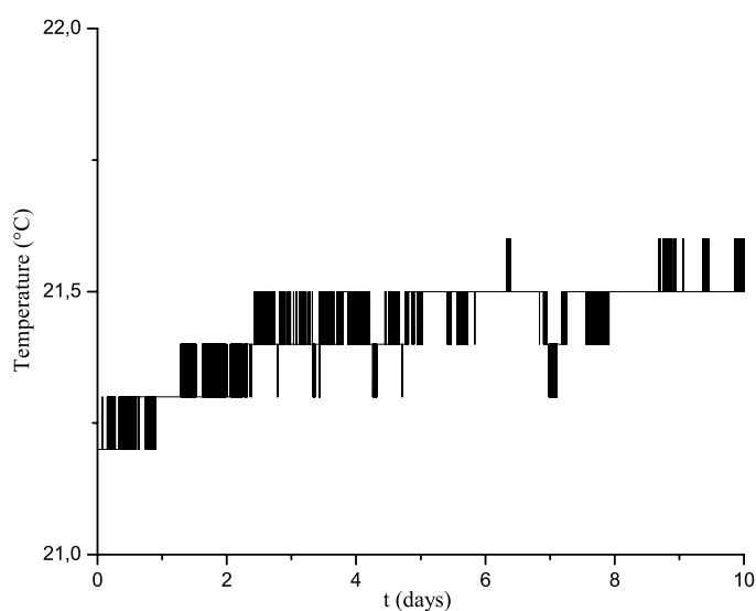
Figure 3. Typical temperature fluctuations of the sample for an acceptable measurement. Temperature data for the measurement results are presented in figure 4. Successive values are connected with a straight line. The precision of the digital thermometer is 0.1^{\circ}\text{C} .
